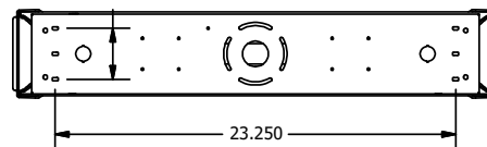
2' End Dimensions
