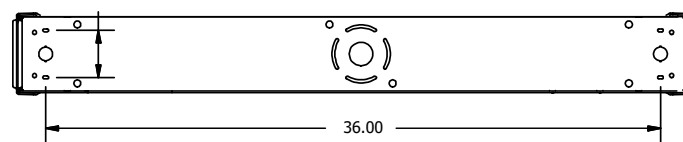
3' End Dimensions
